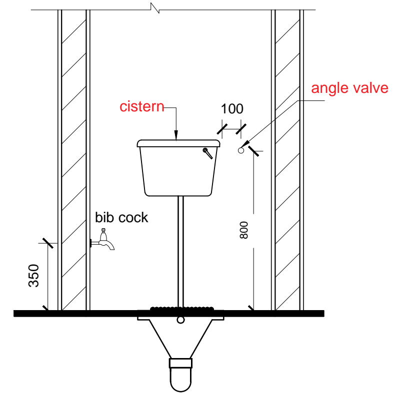
Pan( Front Elevation)
