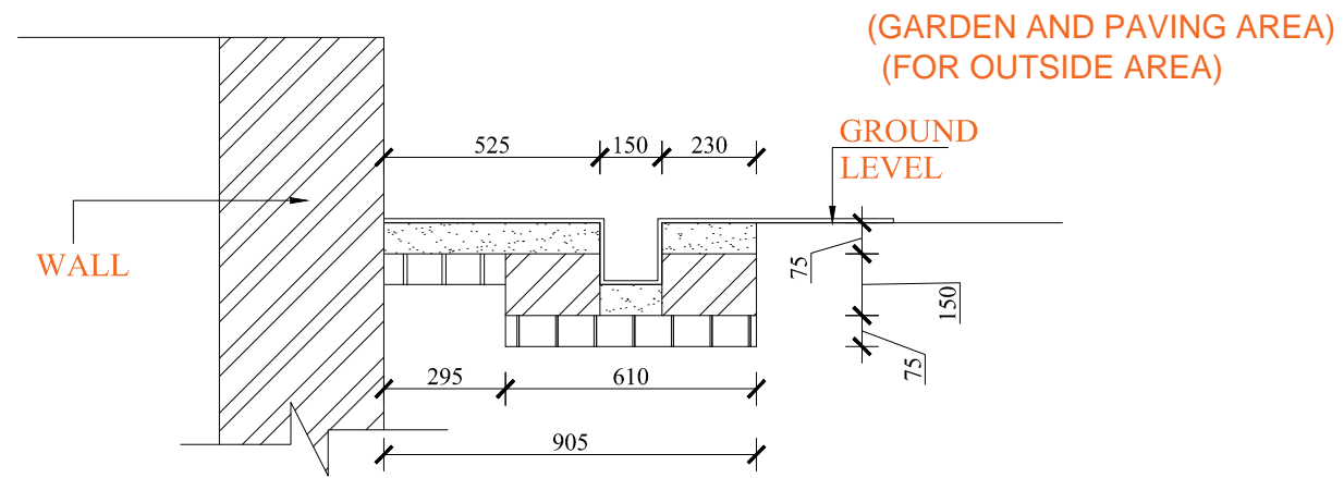
Apron Drain Section
